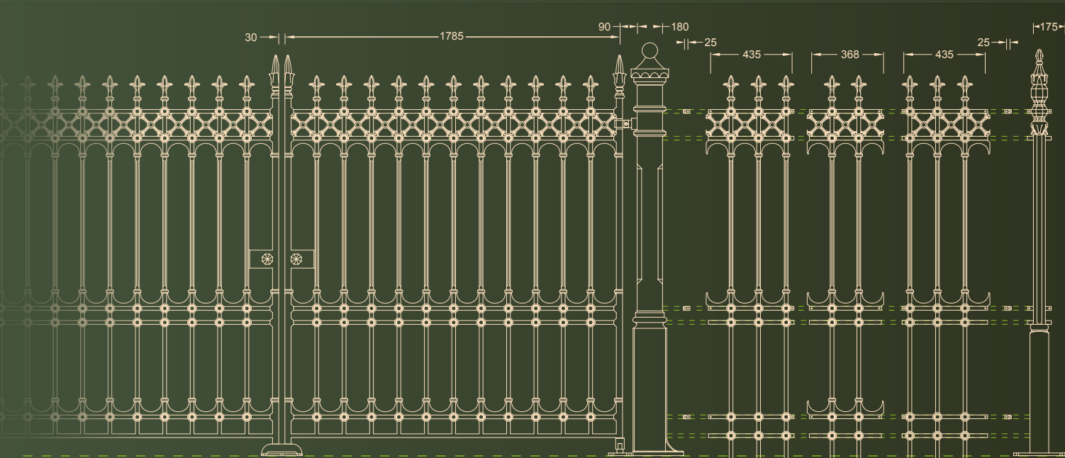
PL1270 - Pillar gate post plate (x2) GL1270 - Driveway gates (x2) RL1570 - Full height railing panel (x2) RL1570J - Full height joining panel (x1) P11570L - Full height intermediate railing post (x1) & End Bracket (x6)
