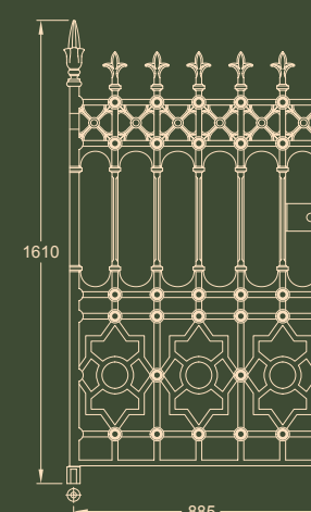
GW3050 Stewart pedestrian gate (3 x 5.5ft, 117kg)
