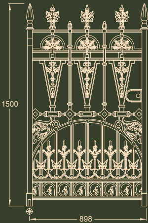
GG3050 Gilberton pedestrian gate leaf (3 x 5ft, 128kg)
