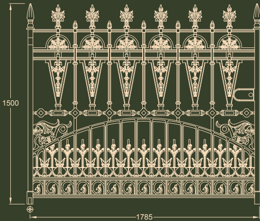
GG1250 Gilberton driveway gate leaf (6 x 5ft, 464kg)
