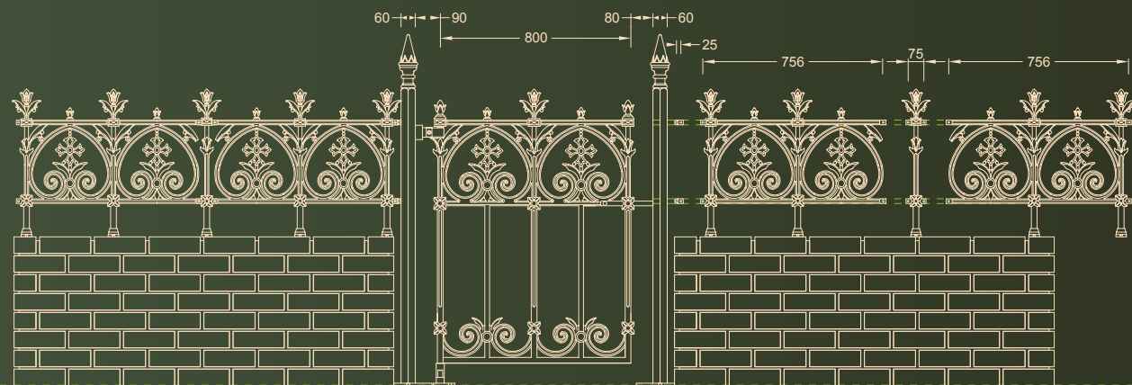
PT3040 - Pillar gate post plate (x2) GT3040 - Eglington Pedestrian gate (x1) RT2010 - Eglington railing panel (x4) RW1050J - Englington joining panel (x2) & End Bracket (x4)
