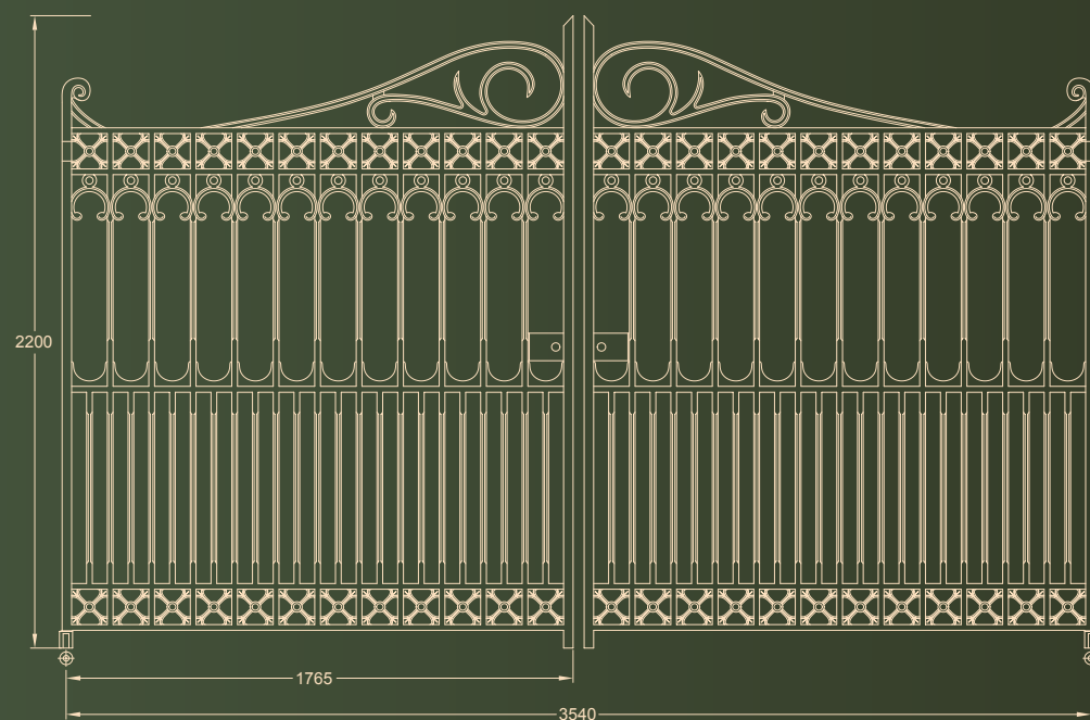
GY1270 Argyle driveway gate leaf (6 x 7ft, 620kg)
