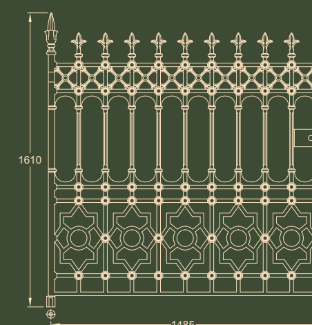
GW1050 Stewart driveway gate leaf (5 x 5.5ft, 370kg)
