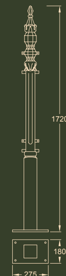
P11050W Stewart full height intermediate railing post (38.5kg)
