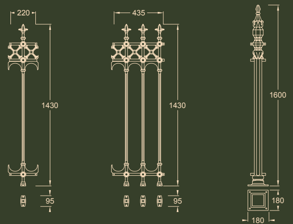
RL1045F Stirling half height joining panel (27kg) RL1545F Stirling half height railing panel (33kg) P11545L Stirling half height intermediate railing post (40kg)
