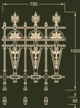
RG1530F Gilberton railing panel (40kg)
