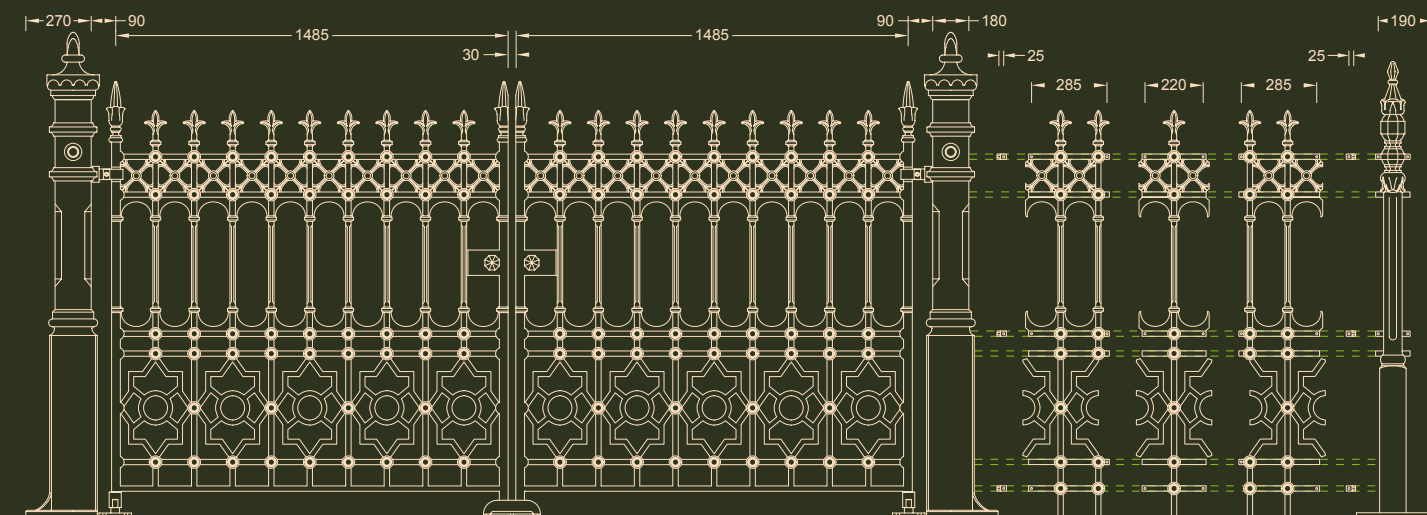
PW1250 - Pillar gate post plate (x2) GW1050 - Driveway gates (x2) RW1050 - Full height railing panel (x2) RW1050J - Full height joining panel (x1) P11050W - Full height intermediate railing post (x1) & End Bracket (x6)
