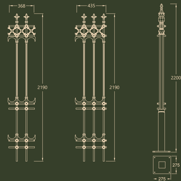
RL1570J Stirling full height joining panel (18kg) RL1570 Stirling full height railing panel (24kg) P11570L Stirling full height intermediate railing post (38.5kg)
